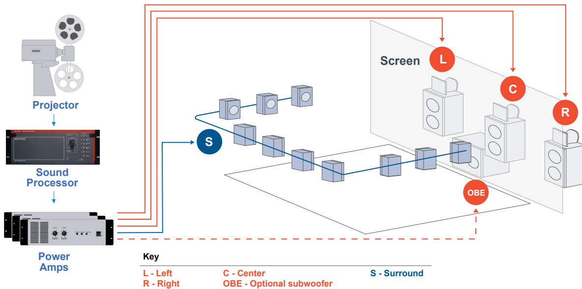
Figure 1.1 Dolby Surround
