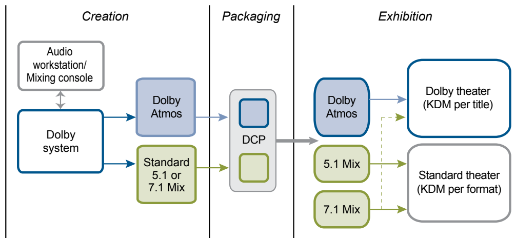
Figure 2.4 Cinema Audio Workflow
