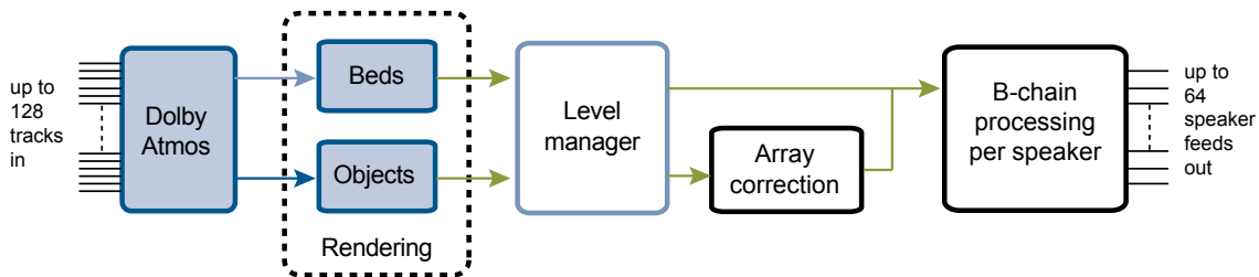
Figure 2.3 Block Diagram of Dolby Atmos Rendering
