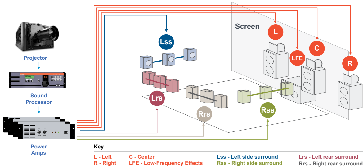
Figure 1.3 Dolby Surround 7.1
