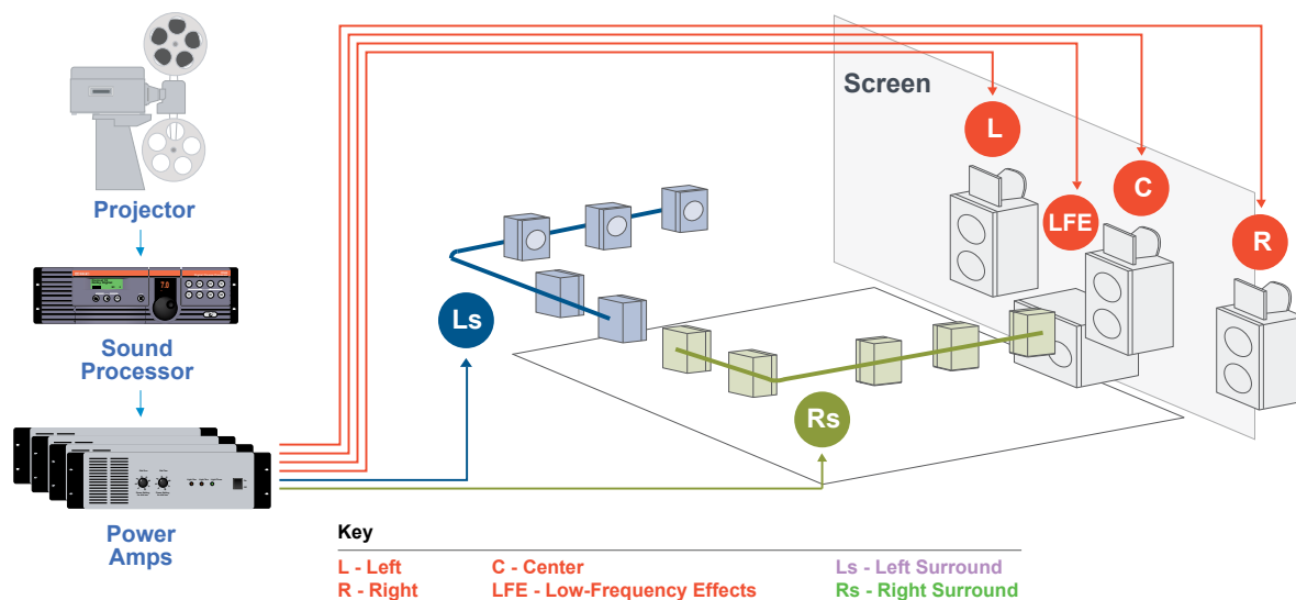
Figure 1.2 Dolby Digital
