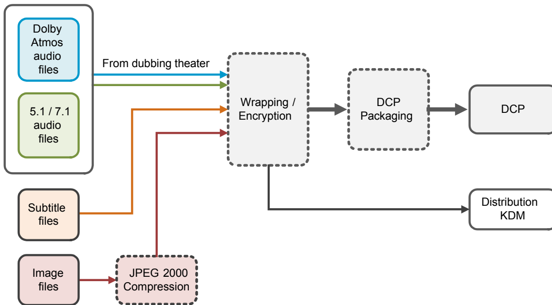
Figure 4.1 Digital Cinema Packaging Workflow
