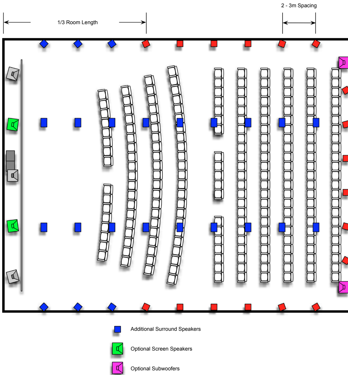
Figure 5.1 Recommended Speaker Locations
