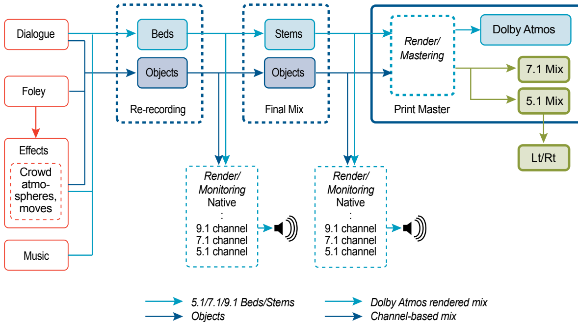
Figure 3.1 Dolby Atmos Audio Post Workflow
