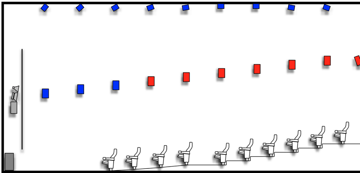
Figure 5.3 Recommended Side Wall and Ceiling Speaker Locations
